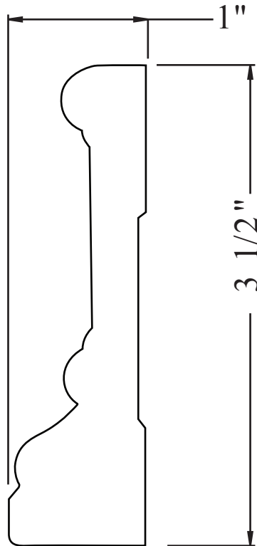
PL1244-25CA 1" x 3 1/2" FULL SCALE
