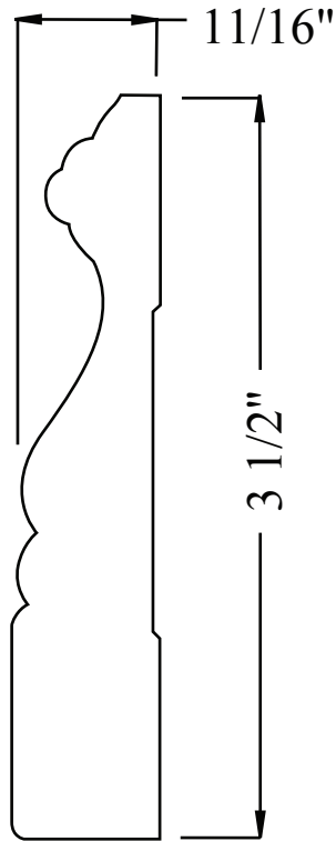
PL155-17CA 11/16" x 3 1/2" FULL SCALE
