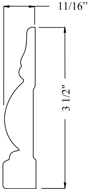
PL165-17CA 11/16" x 3 1/2" FULL SCALE
