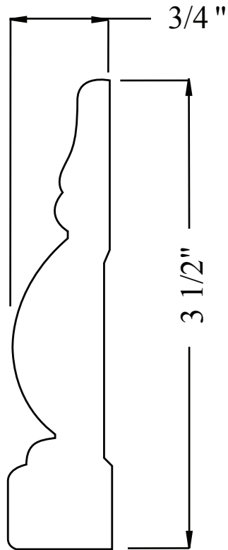
PL165-19CA 3/4" x 3 1/2" FULL SCALE
