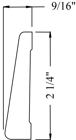
PL324-15CA 9/16" x 2 1/4" FULL SCALE
