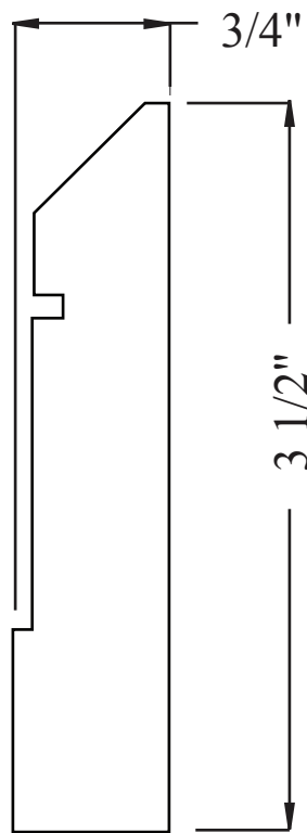
PL005-19CA 3/4" x 3 1/2" FULL SCALE
