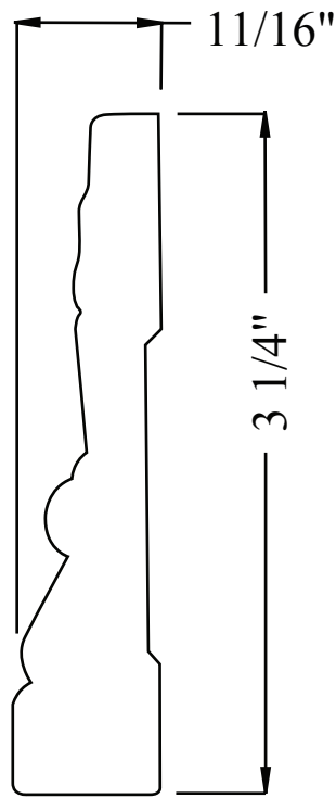
PL009-17CA 11/16'' \times 3 \frac{1}{4}'' FULL SCALE
