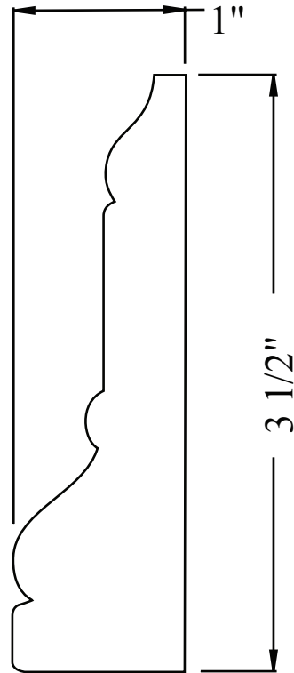
PL123-25CA 1" x 3 1/2" FULL SCALE
