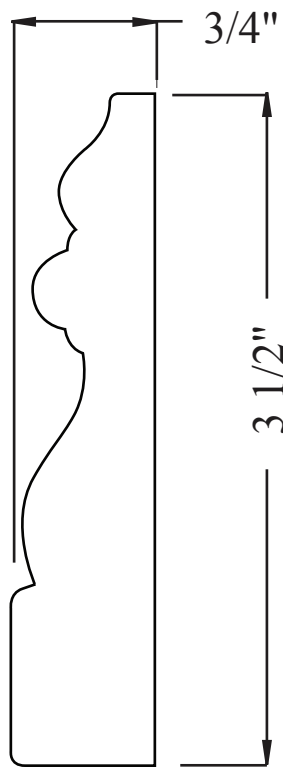
PL129-19CA 3/4" x 3 1/2" FULL SCALE
