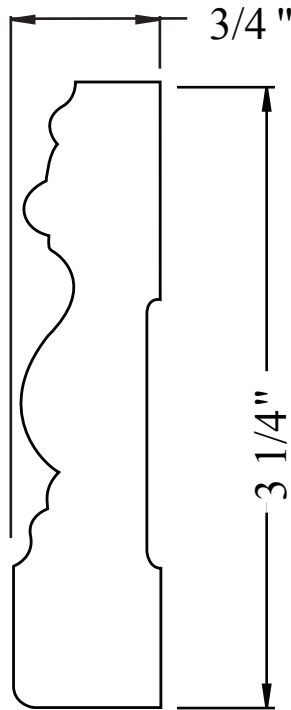
PL325-19CA 3/4" x 3 1/4" FULL SCALE
