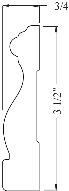
PL350-19CA 3/4" x 3 1/2" FULL SCALE
