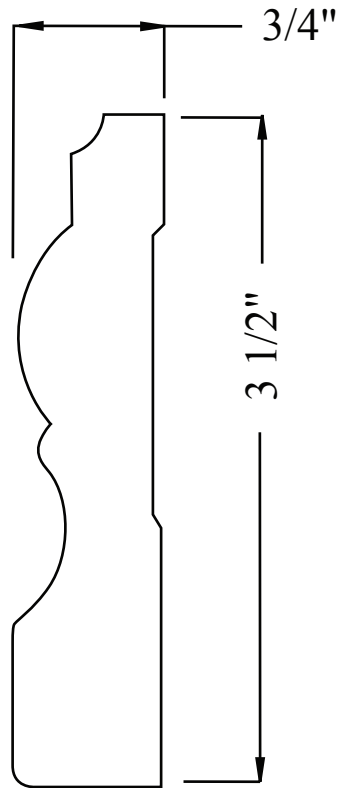
PL352-19CA 3/4" x 3 1/2" FULL SCALE
