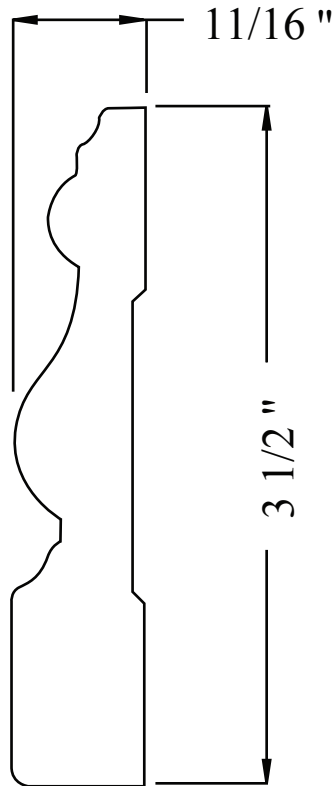
PL353-17CA 11/16" x 3 1/2" FULL SCALE
