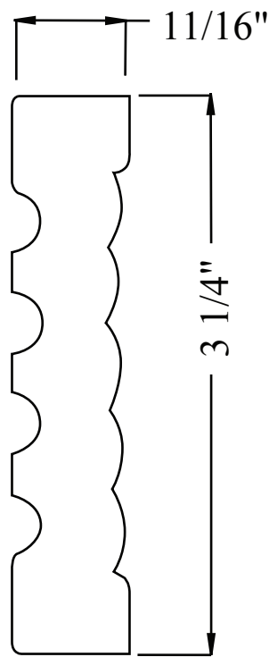
PL401-17CA 11/16" x 3 1/4" FULL SCALE
