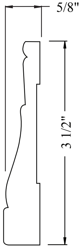
PL447-15CA 5/8" x 3 1/2" FULL SCALE
