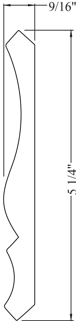
PL045-14CR 9/16" x 5 1/4" FULL SCALE
