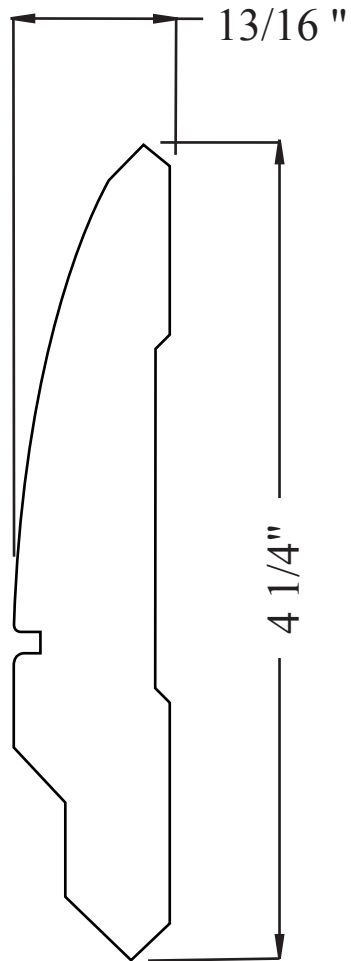
PL001-21CR 13/16" x 4 1/4" FULL SCALE
