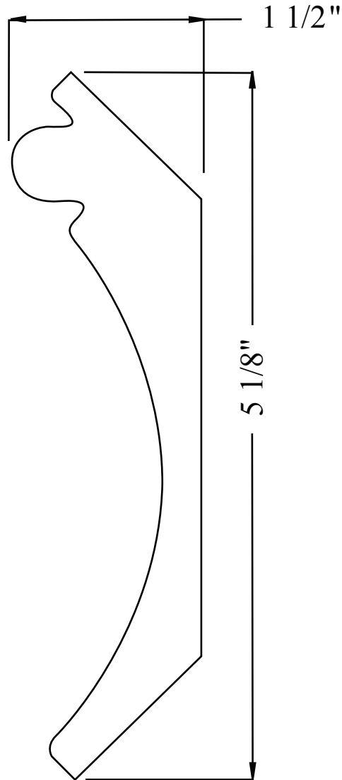
PL016-38CR 1 1/2" x 5 1/8" FULL SCALE
