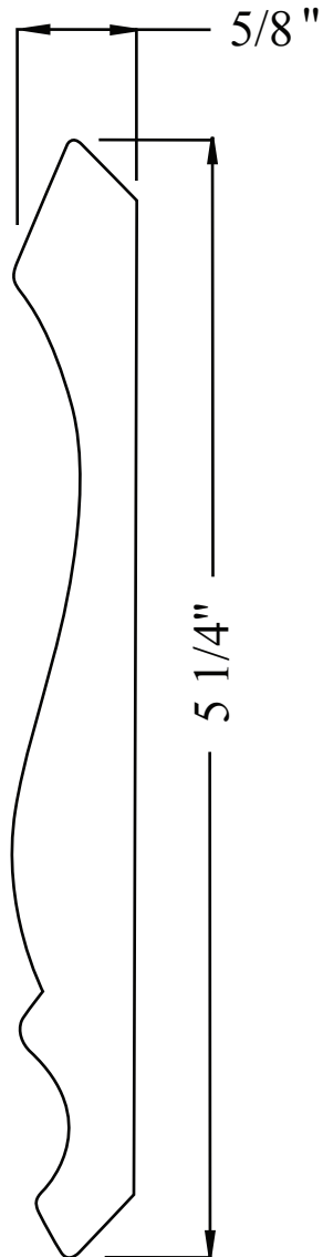
PL044-15CR 5/8" x 5 1/4" FULL SCALE
