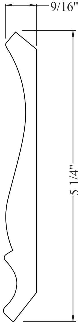
PL056-14CR 9/16" x 5 1/4" FULL SCALE
