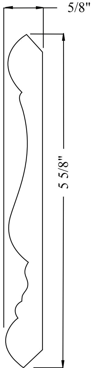
PL141-15CR 5/8" x 5 5/8" FULL SCALE
