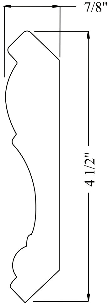
PL185-22CR 7/8" x 4 1/2" FULL SCALE
