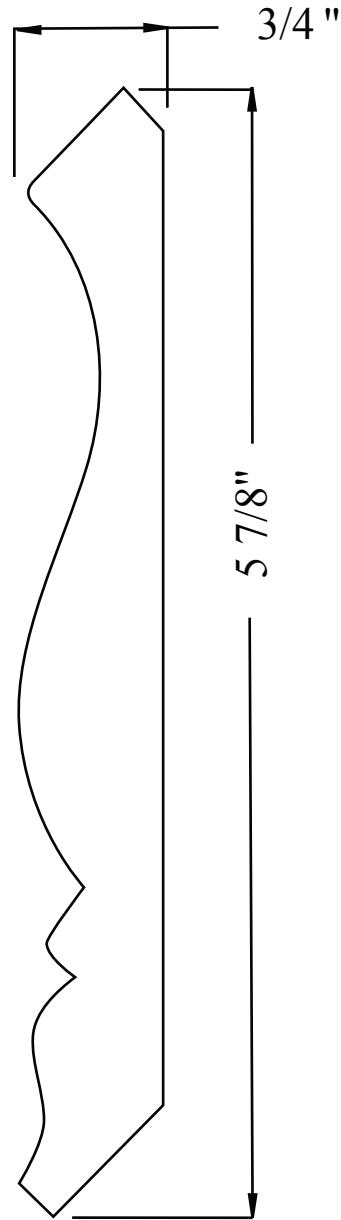
PL417-19CR 3/4" x 5 7/8" FULL SCALE
