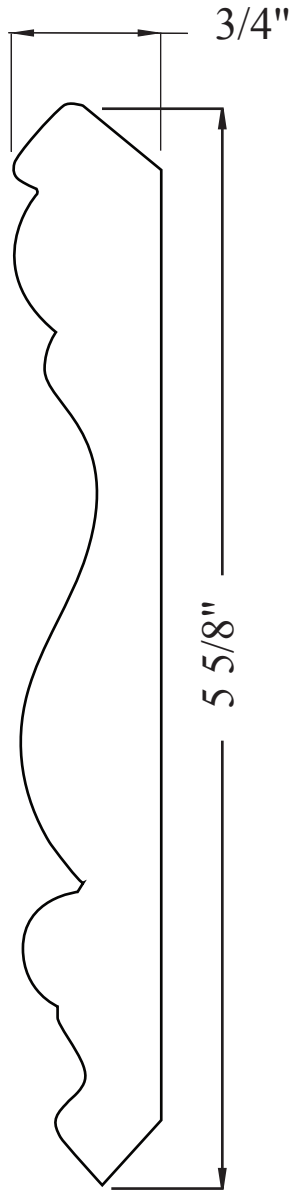
PL550-19CR 3/4" x 5 5/8" FULL SCALE
