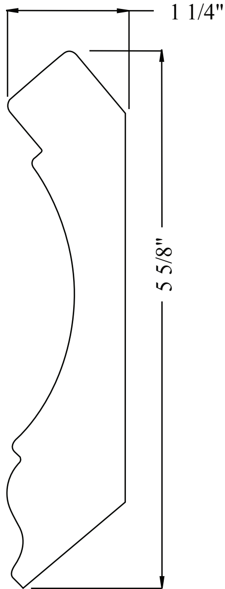
PL562-32CR 1 1/4" x 5 5/8" FULL SCALE
