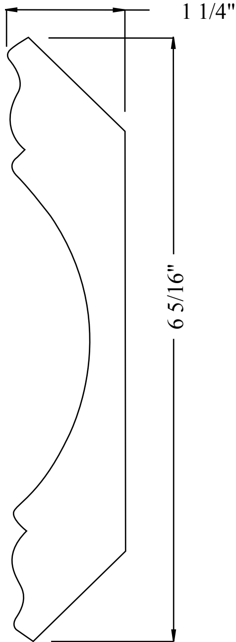
PL625-32CR 1 1/4" x 6 5/16" FULL SCALE
