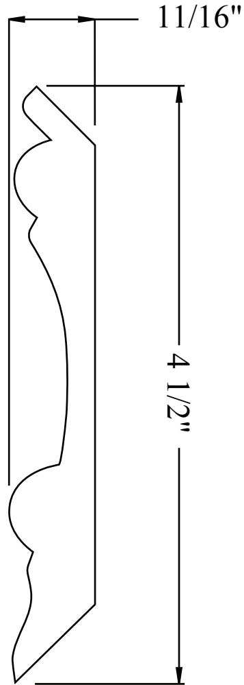
PL824-17CR 11/16" x 4 1/2" FULL SCALE
