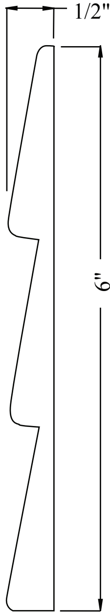
PL006-12FL 1/2" x 6" FULL SCALE
