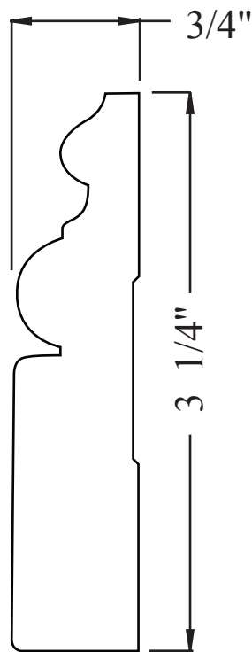
PL325-19CE 3/4" x 3 1/4" FULL SCALE
